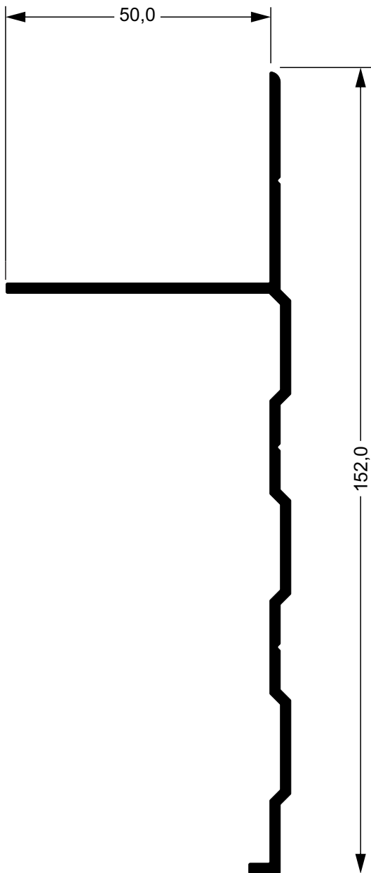
29112 1,138 kg/m Longarina Inferior
